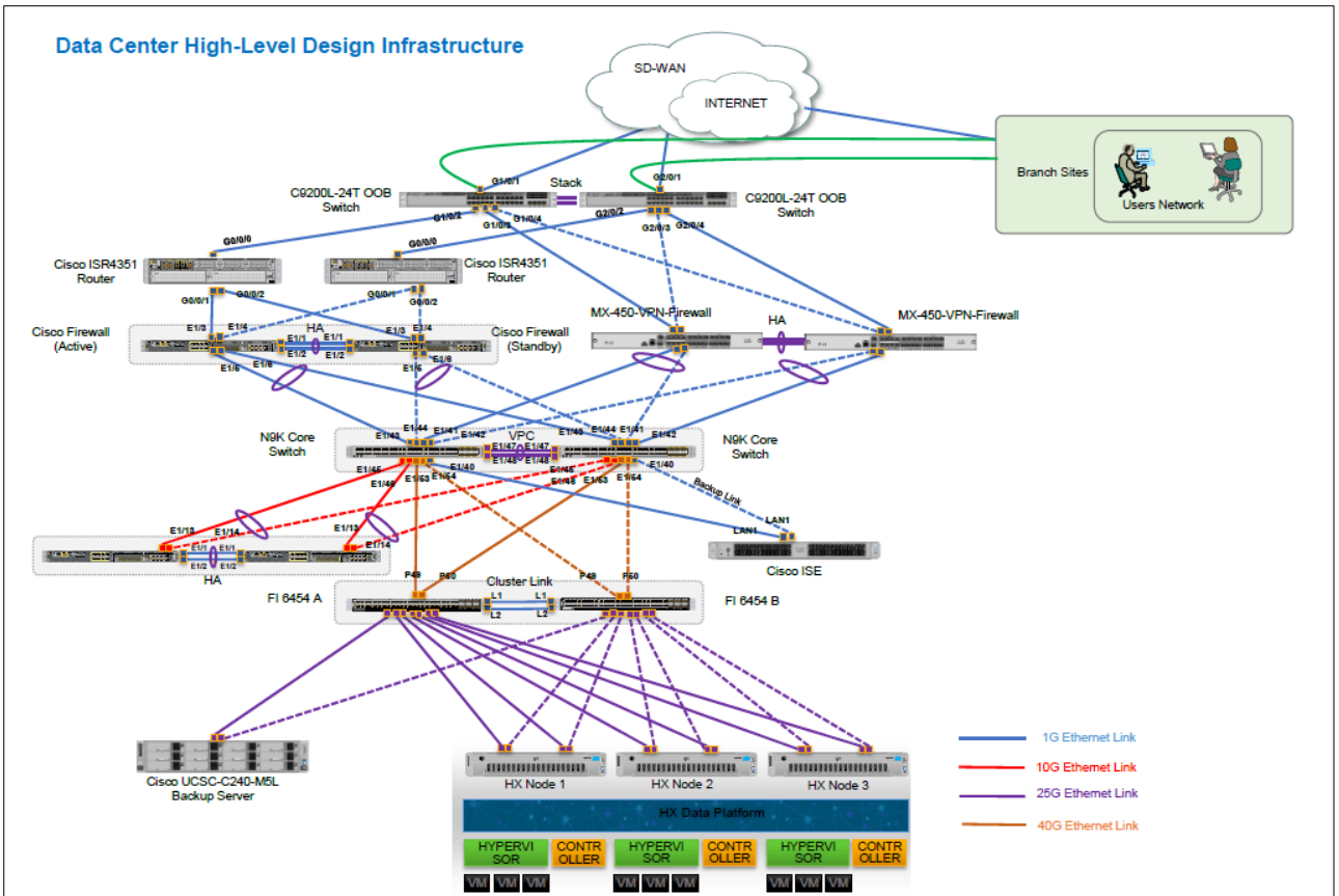
ပုံ (4) - Data center ၏ High Level design ပုံစံ (as Reference)
